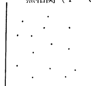
無相関 ( r = 0 )
