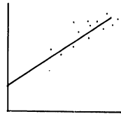
順相関 ( r > 0 )
